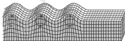
Unde Rayleigh-R
