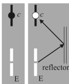
Fig. 3.64. Reflexia undelor electromagnetice
