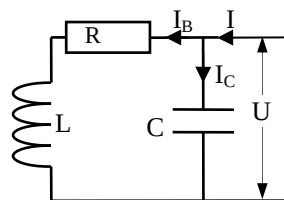
Fig. 3.41. Circuit paralel LC real
