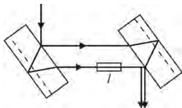
Fig. 4.30. Interferometrul Jamin
